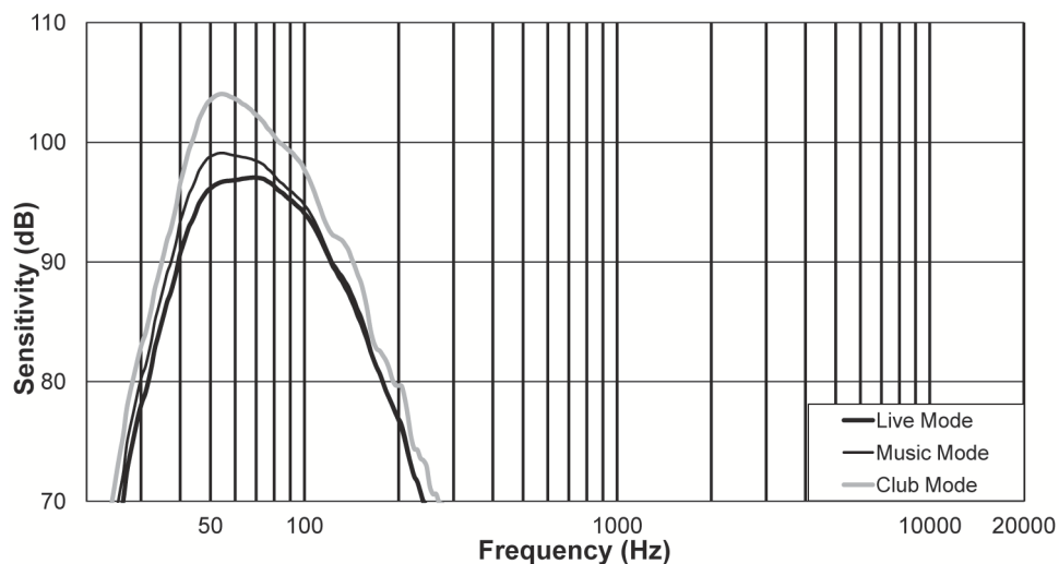
Figure 9.4: EKX-18SP Frequency response graph: live, music, and club modes
