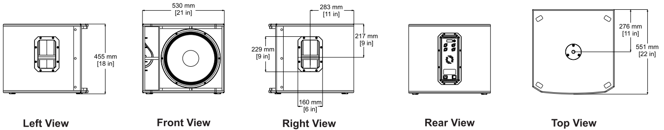
Figure 3.3: EKX-15SP dimensions
