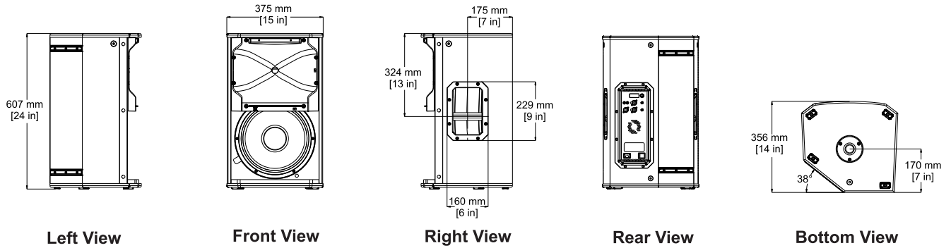
Figure 3.1: EKX-12P dimensions
